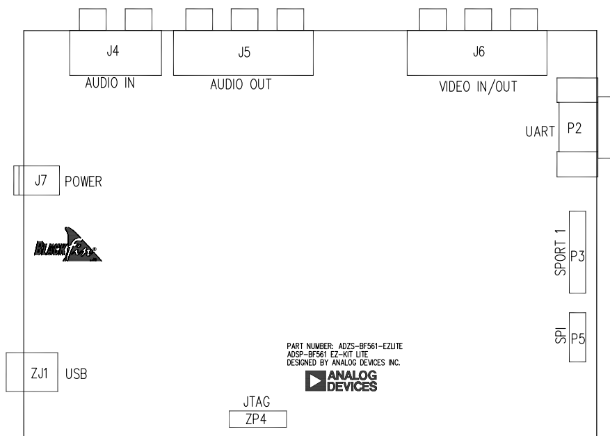
Figure 2-4. Connector Locations
