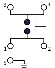
CIRCUIT: SPST ▲
