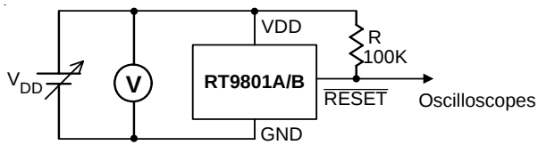
Detection Voltage
