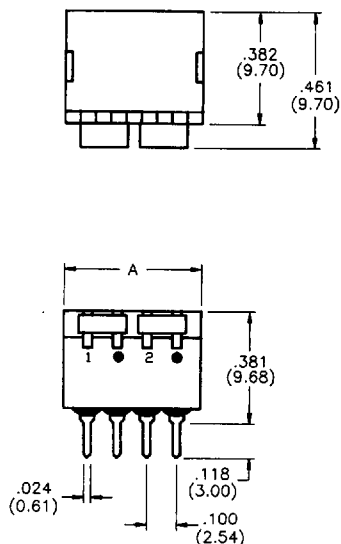
Mechanical Outline
