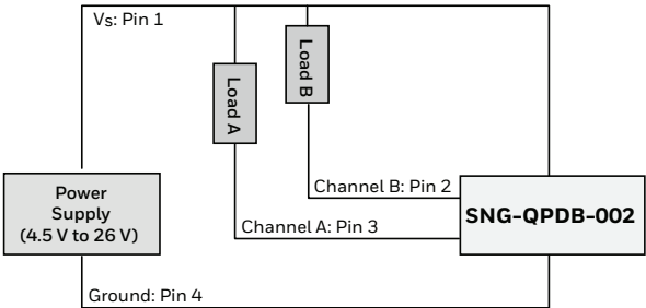
Circuit Diagram
