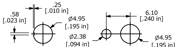
WITH STANDARD LOCKING RING
