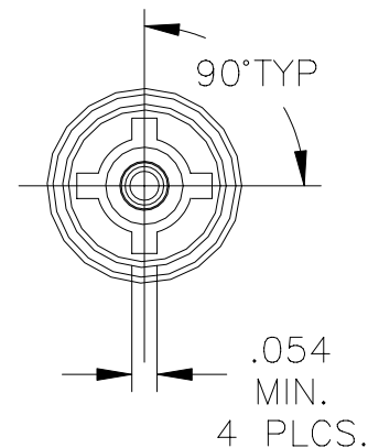
INTERFACE "D" PLUG
