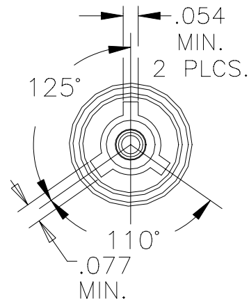
INTERFACE "C" PLUG
