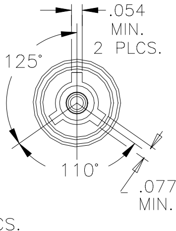
INTERFACE "B" PLUG
