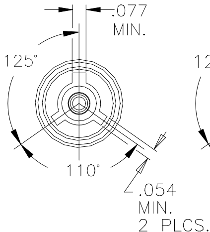
INTERFACE "A" PLUG
