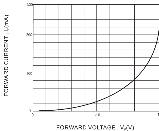
Fig.3 Forward current as a function of forward voltage ; typical values
