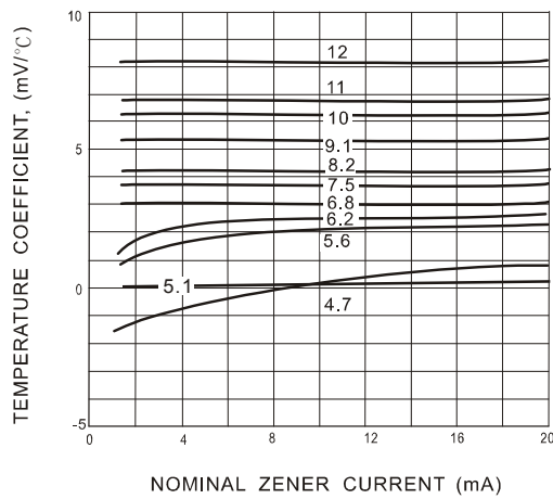
Fig.1 TEMPERATURE COEFFICIENTS AS FUNCTION OF WORKING CURRENT ; TYPICAL VALUES
