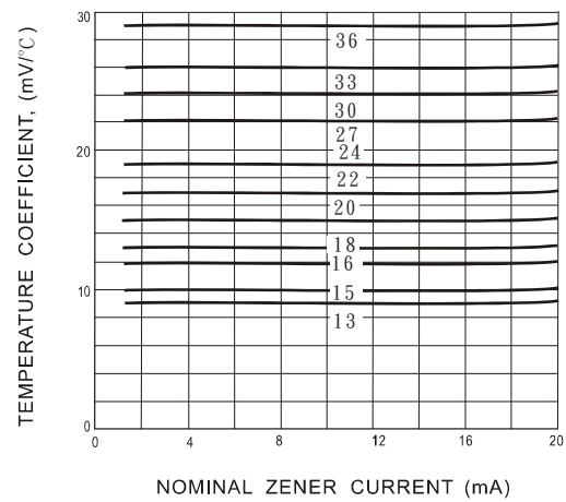
Fig.2 TEMPERATURE COEFFICIENTS AS FUNCTION OF WORKING CURRENT ; TYPICAL VALUES
