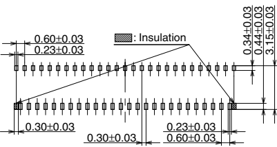
Recommended metal mask pattern Metal mask thickness: When 120μm (Front terminal portion opening area ratio: 96%) (Back terminal portion opening area ratio: 96%)
