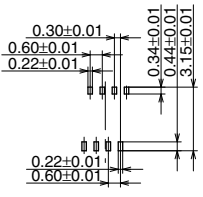
Recommended metal mask pattern Metal mask thickness: When 120μm (Front terminal portion opening area ratio: 96%) (Back terminal portion opening area ratio: 96%)
