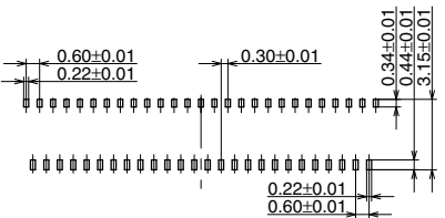
Recommended metal mask pattern Metal mask thickness: When 120μm (Front terminal portion opening area ratio: 96%) (Back terminal portion opening area ratio: 96%)
