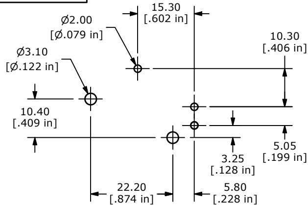
P.C. MOUNTING
