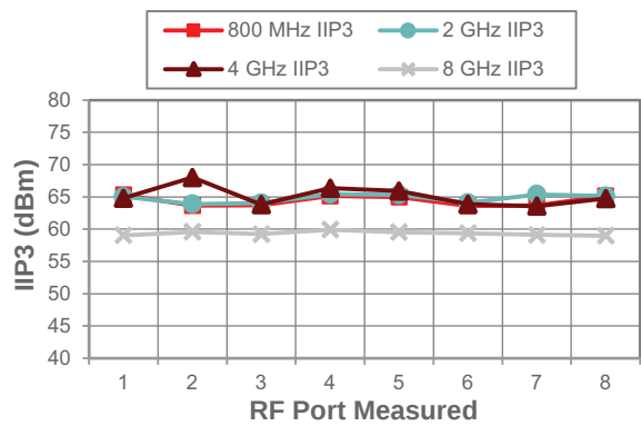
Figure 20 • IIP3 vs. RF Port Measured
