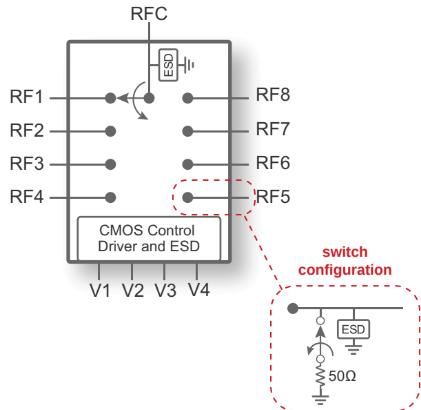
Figure 1 • PE42482 Functional Diagram
