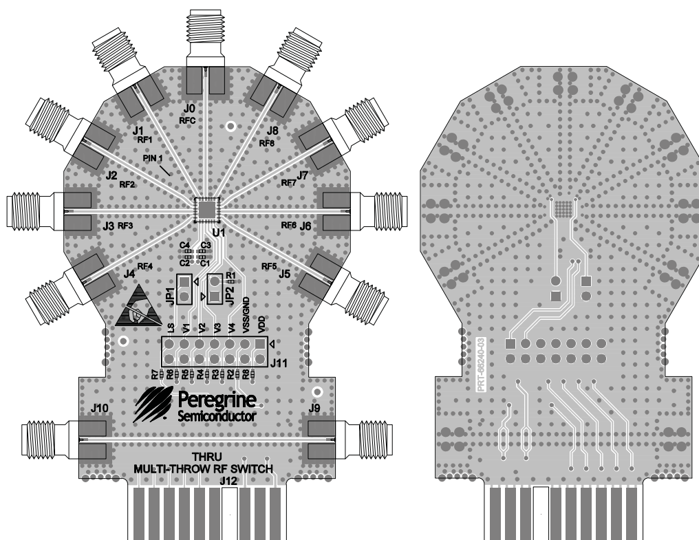
Figure 21 • Evaluation Board Layout for PE42482
