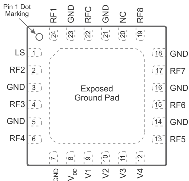
Figure 22 • Pin Configuration (Top View)
