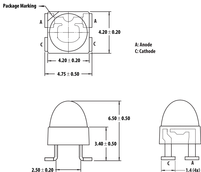
Figure 1: Package Dimensions
