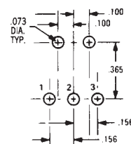
Contacts Make on Opposite Side Toggle Thrown
