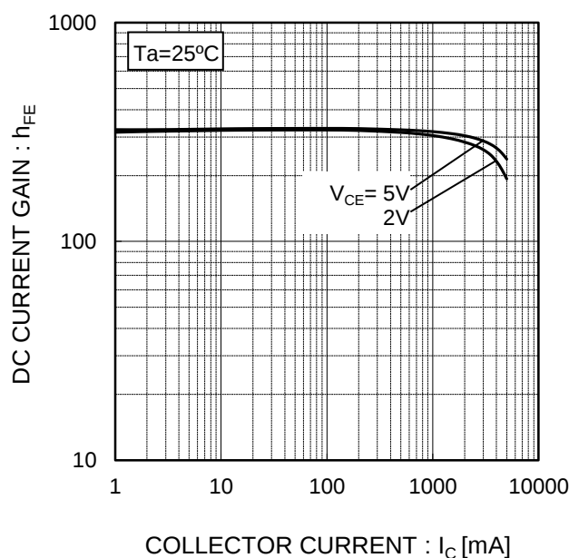
Fig.4 DC current gain vs. output current (II)
