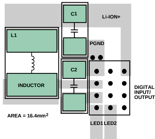
Figure 2. PCB Layout
