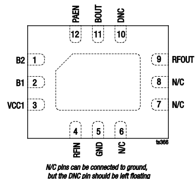
Figure 2. SE2433T Pinout (Top View)
