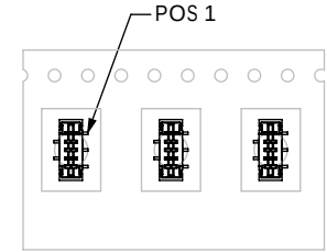
TAPE & REEL VIEW FOR VERTICAL PARTS
