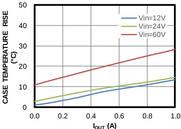
Case Temp Rise vs. Load Current
