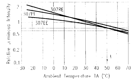
Fig.16 LUMINOUS INTENSITY VS. AMBIENT TEMPERATURE
