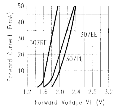
Fig.10 FORWARD CURRENT VS. FORWARD VOLTAGE
