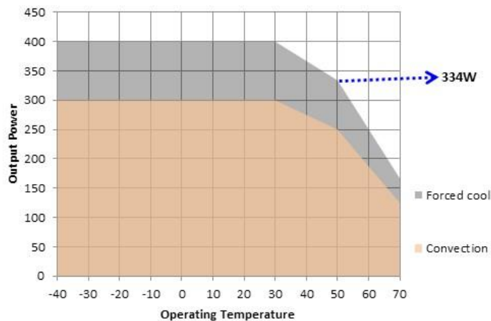
Figure 6. Power Derating Curve 12 V
