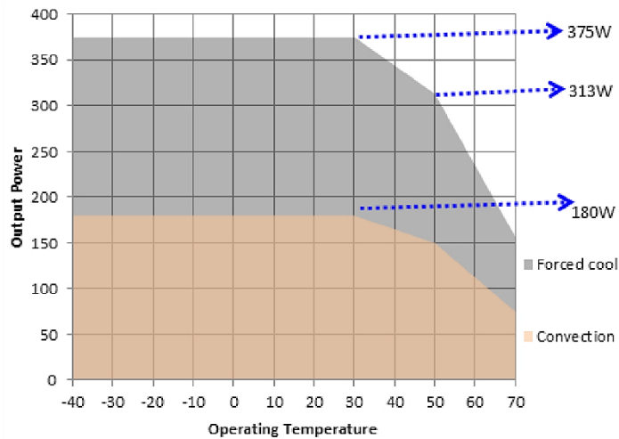
Figure 8. Power Derating Curve 12 V with Plain Cover
