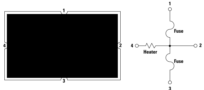
Device Circuit
