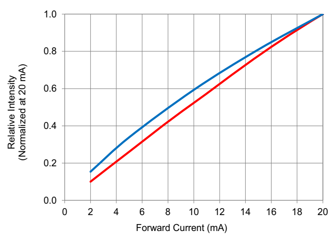
Figure 3: Relative Luminous Intensity vs. Mono Pulse Current
