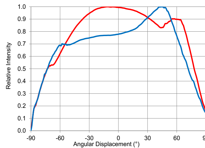
Figure 4: Radiation Pattern
