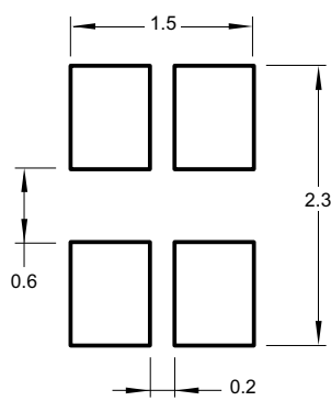
Figure 6: Recommended Soldering Land Pattern
