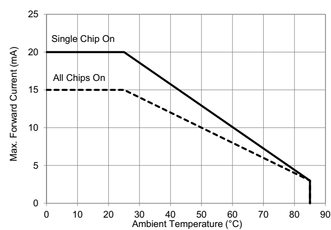
Figure 5: Derating Curve
