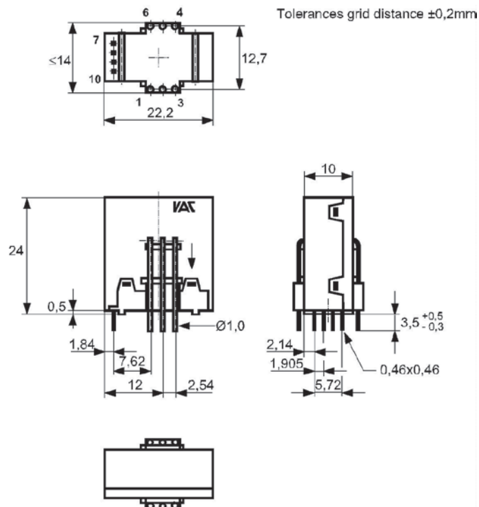
Drawing no. 2
