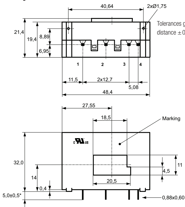
Drawing no. 4
