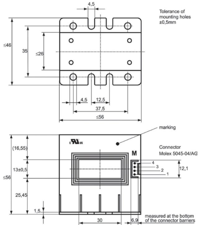
Drawing no. 1
