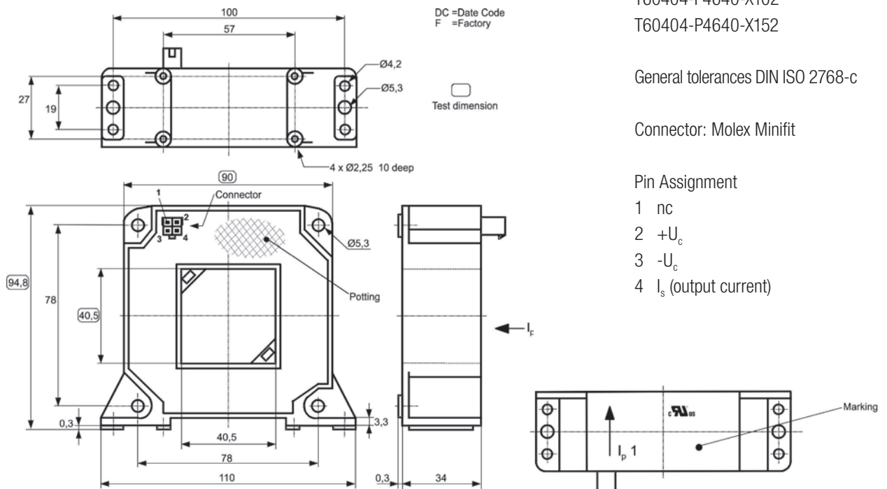
Drawing no. 4
