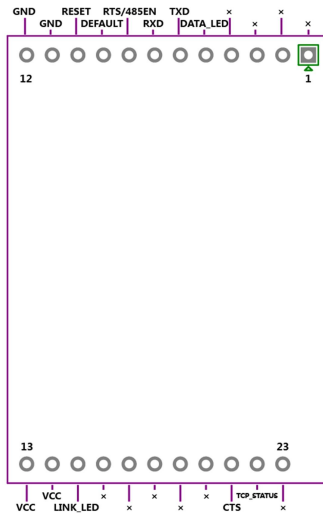
Figure 2-2 W7500S2E-R1 pinout
