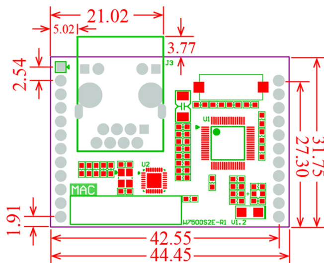
Figure 1-3 W7500S2E-R1 dimension - top view
