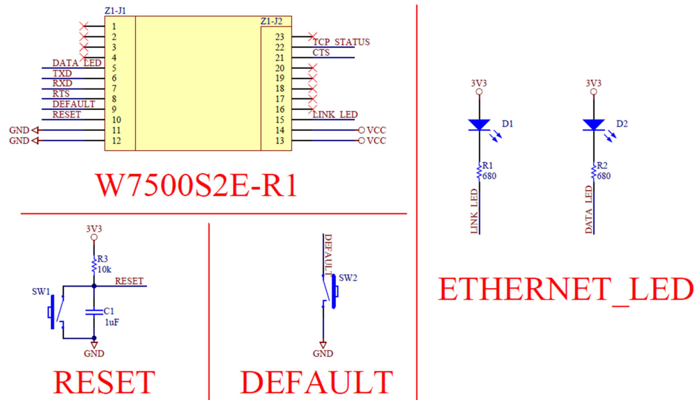
Figure 2-5 W7500S2E-R1 reference schematic
