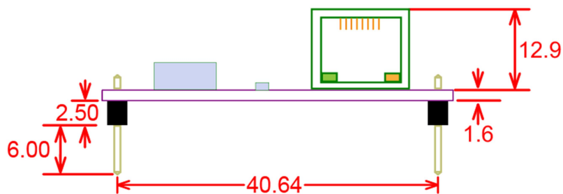
Figure 1-4 W7500S2E-R1 dimension - side view
