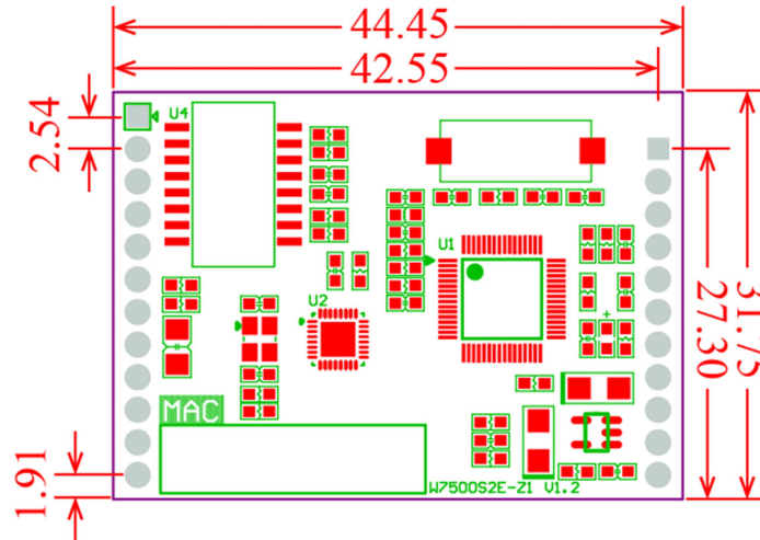
Figure 1-1 W7500S2E-Z1 dimension - top view
