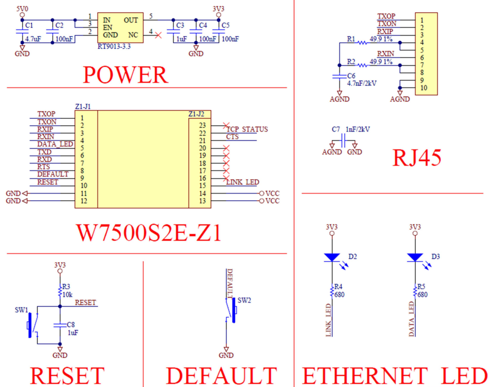
Figure 2-4 W7500S2E-Z1 reference schematic
