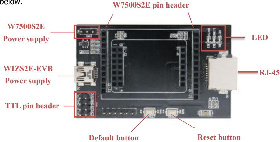
Figure 2-3 WIZS2E breakout board
