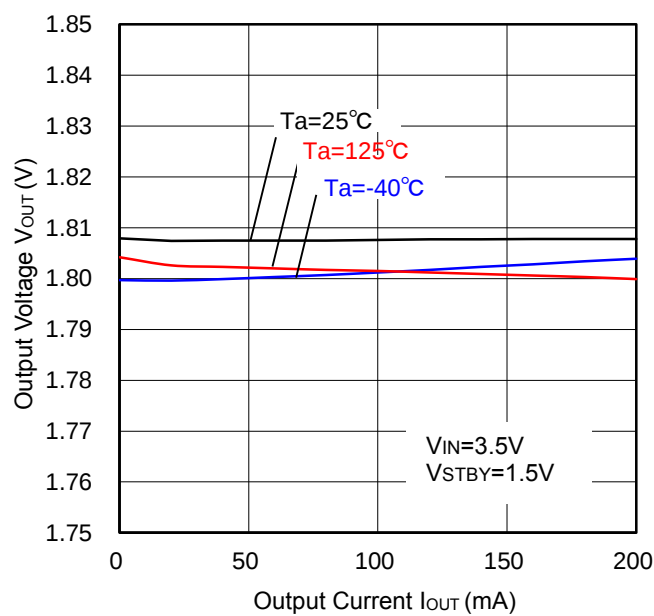
Figure 6. Load Regulation
