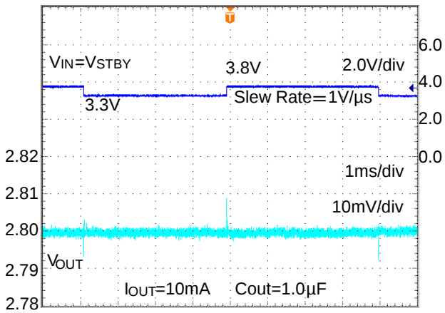
Figure 39. Line Transient Response (3.3V to 3.8V)
