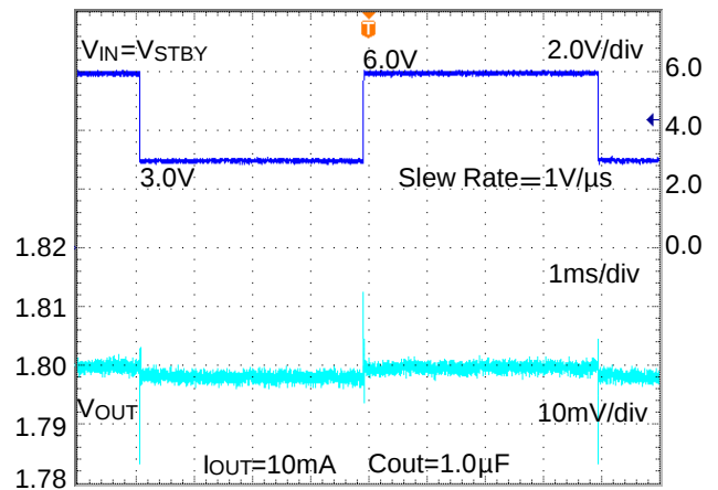
Figure 19. Line Transient Response (3.0V to 6.0V)
