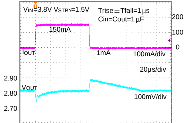
Figure 38. Load Response (1mA to 150mA)
