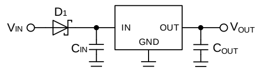
Figure 55. Protection against Reverse Polarity 1
