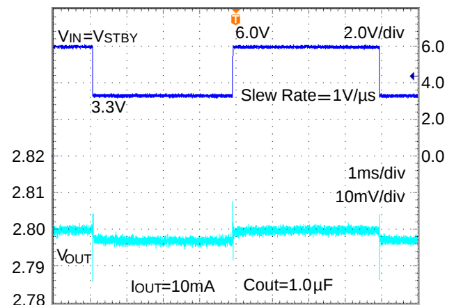
Figure 40. Line Transient Response (3.3V to 6.0V)
