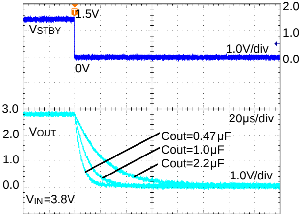
Figure 44. Discharge Time ( R_{OUT} = 14 \Omega )
