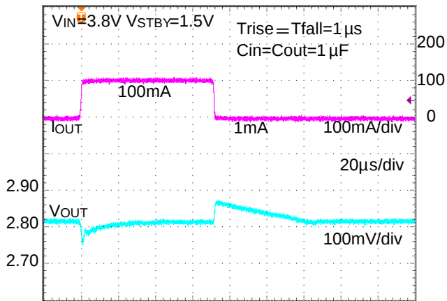
Figure 37. Load Response (1mA to 100mA)
