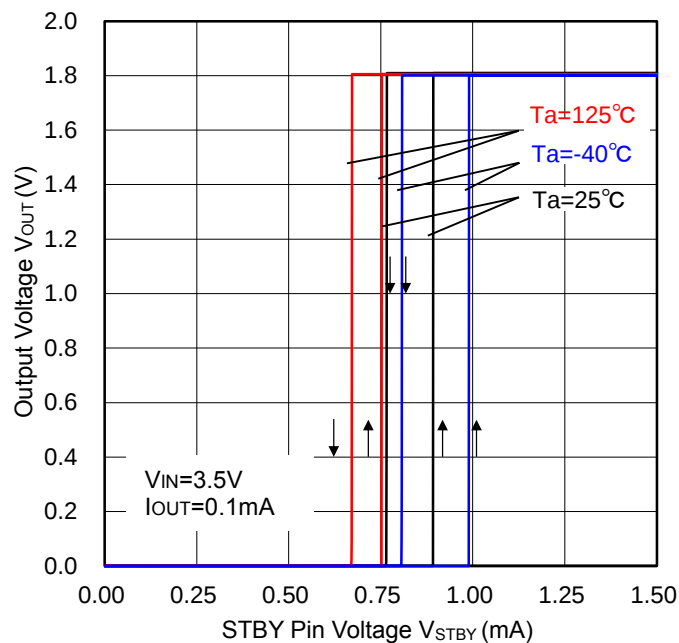
Figure 11. STBY Threshold
