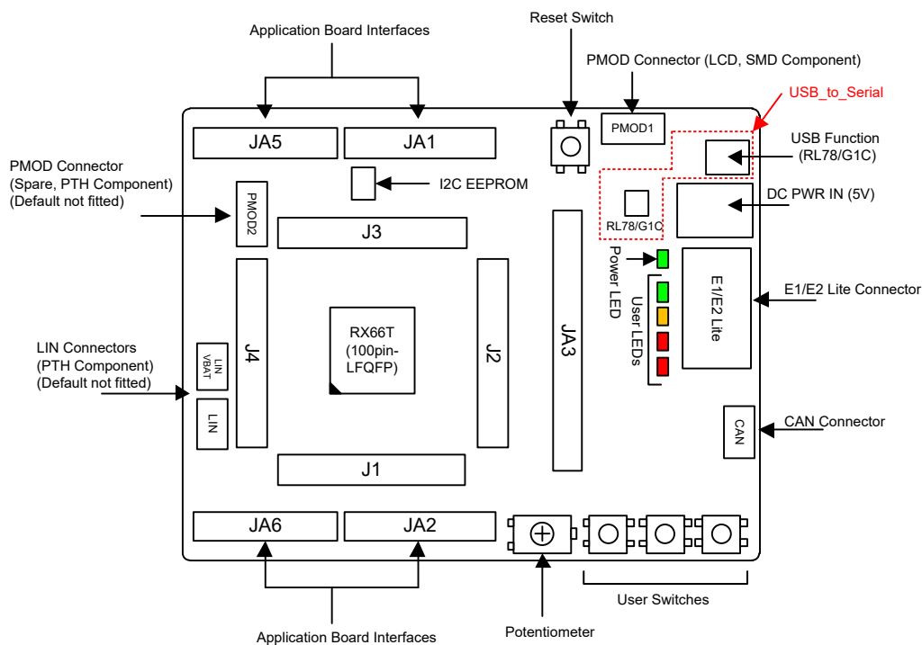
Figure 3-1: Board Layout
