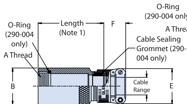
Direct-Coupling Style 1
