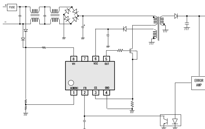
Figure 1. Application circuit
