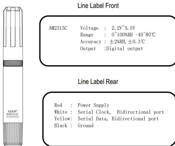
Figure 13. Sensor laser marking
