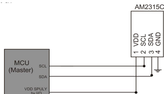
Figure 8. Typical application circuit
