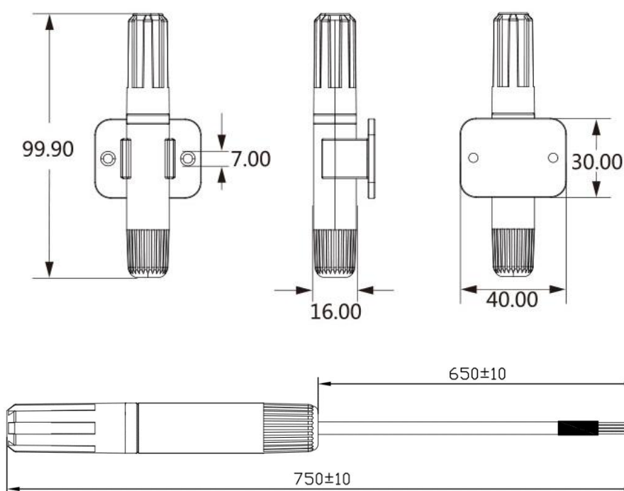
Figure 12. AM2315C sensor encapsulation (unit: mm not specified tolerance: \pm 0.2 mm)
