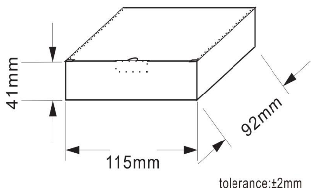
Figure 15. Schematic diagram of packaging
