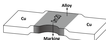
Shunt structure
