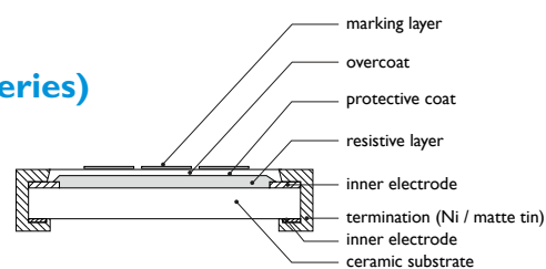
Cross section of RL / PT series
