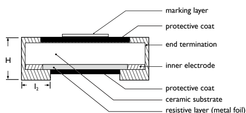
Cross section of wide termination series
