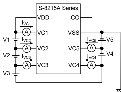
Figure 8 Test Circuit 4
