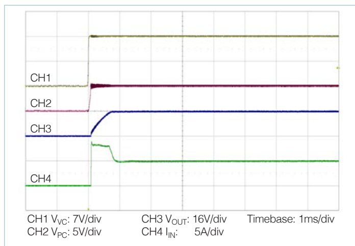
Figure 14 — Start up from application of V_C ; V_{IN} pre-applied C_{OUT} = 800\mu\text{F}
