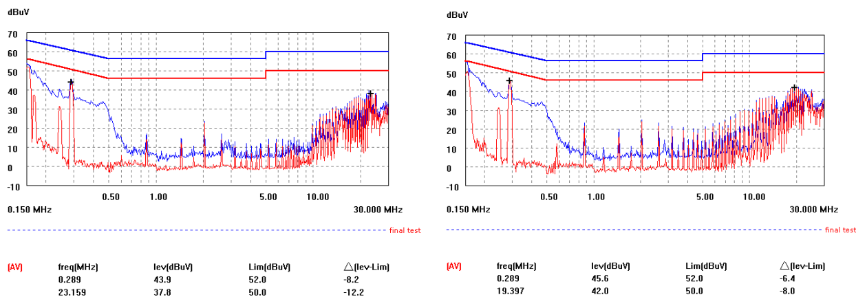
Figure 23. EMC Filter
