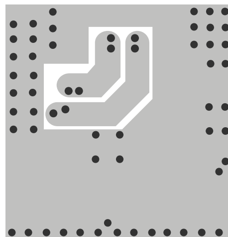
Figure 3 — Layer 2
