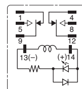
DPDT
