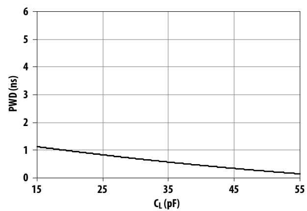
Figure 8: Typical Pulse Width Distortion vs Load Capacitance at 3.3V Supply Voltage
