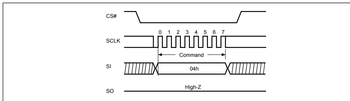
Figure 3. Write Disable (WRDI) Sequence (Command 04h)
