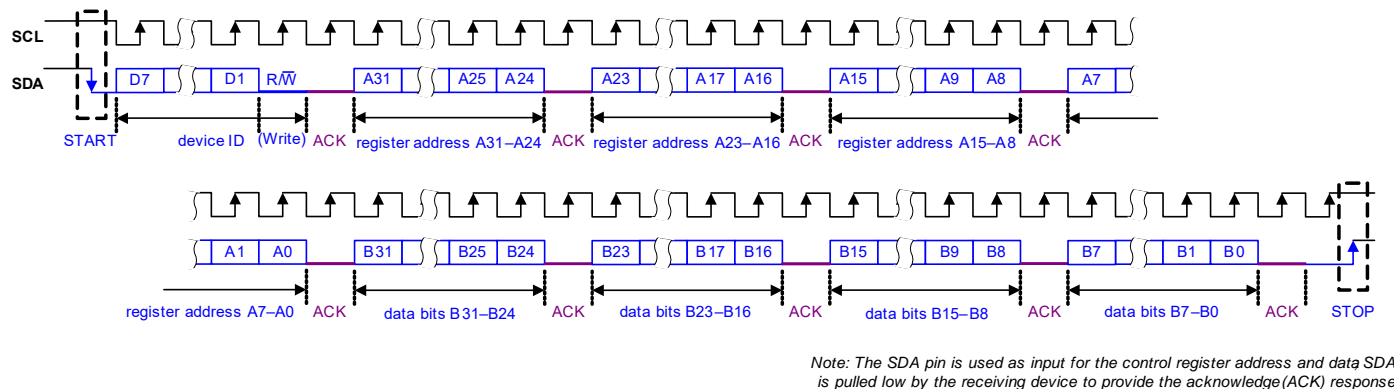
Figure 4-59. Control Interface I 2 C Register Write
