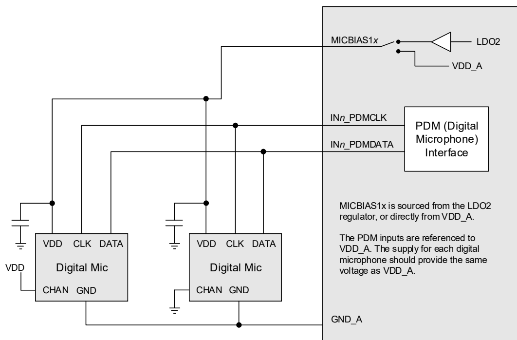
Figure 4-10. DMIC Input
