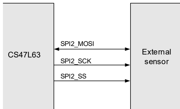
Figure 4-33. 3-Wire Mode
