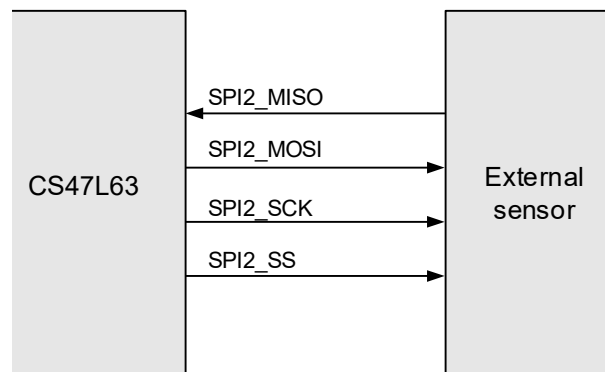
Figure 4-34. 4-Wire Mode
