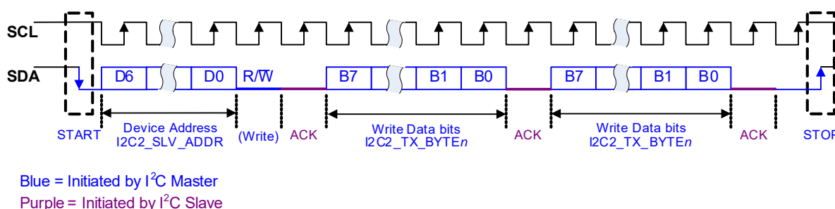
Figure 4-30. Master I 2 C Write
