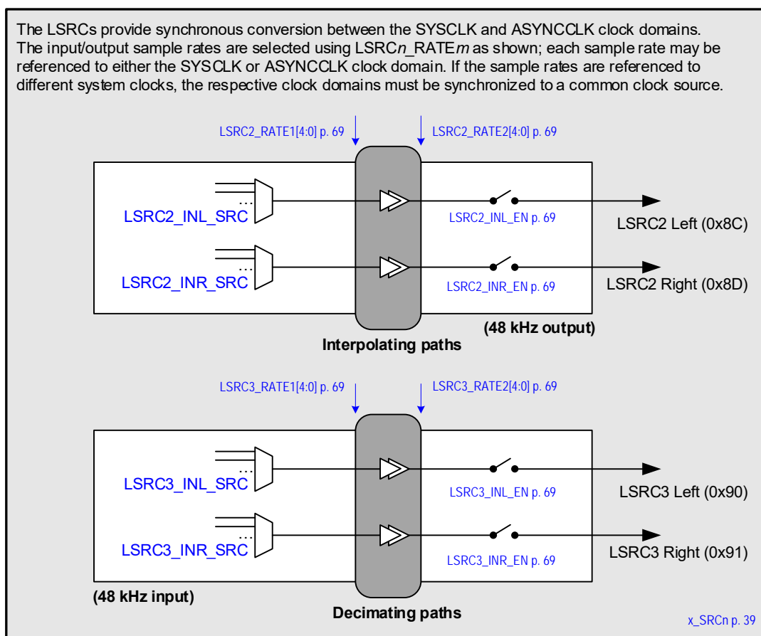
Figure 4-26. Low-Power Sample-Rate Converters (LSRCs)
