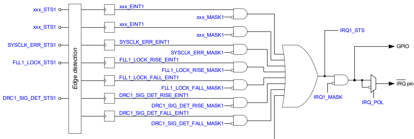
Figure 4-56. Interrupt Controller
