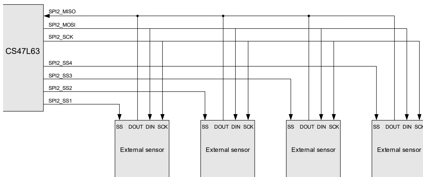
Figure 4-35. Multiple-Slave Configuration
