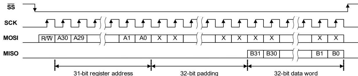
Figure 4-58. Control Interface SPI Register Read
