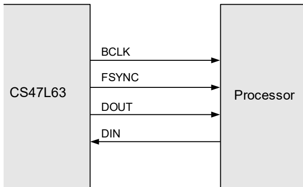
Figure 4-39. Master Mode
