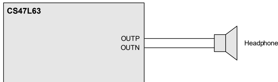
Figure 4-53. Headphone Connection
