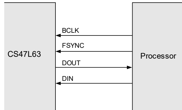
Figure 4-40. Slave Mode
