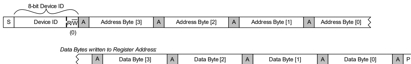
Figure 4-61. Single-Register Write to Specified Address
