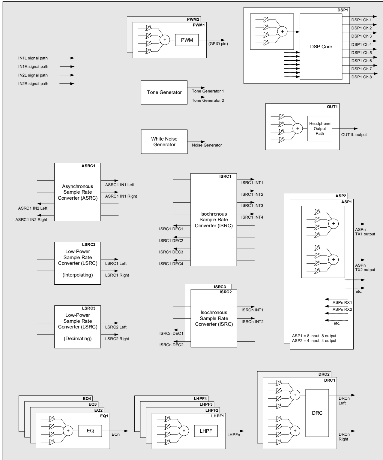
Figure 4-12. Digital Core
