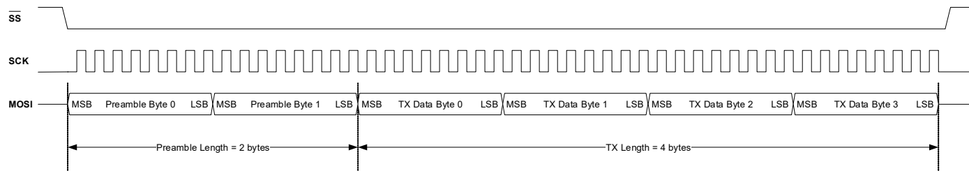
Figure 4-37. SPI Master Write, with Preamble
