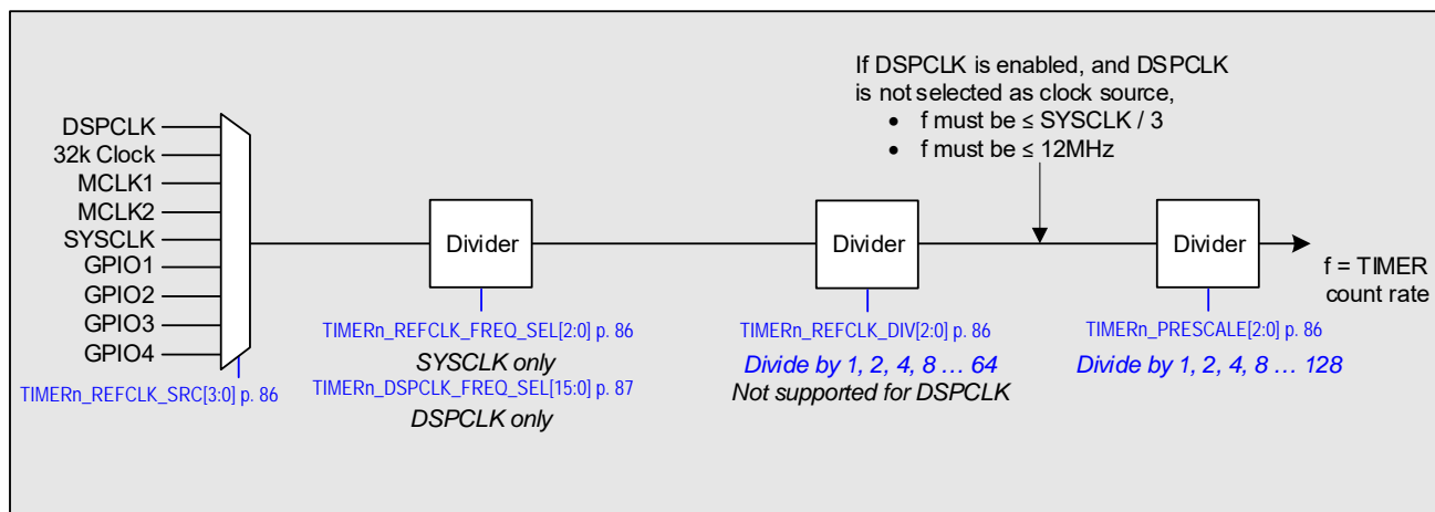
Figure 4-28. General-Purpose Timer
