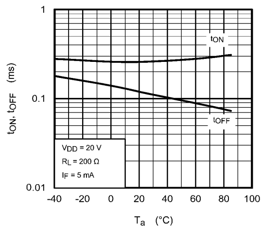
Fig. 16.8 t_{ON}, t_{OFF} - T_a
