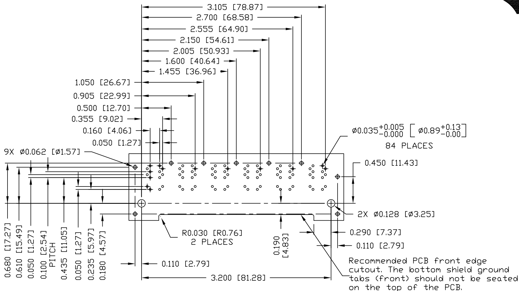
SUGGESTED PCB FOOTPRINT (COMPONENT SIDE VIEW)
