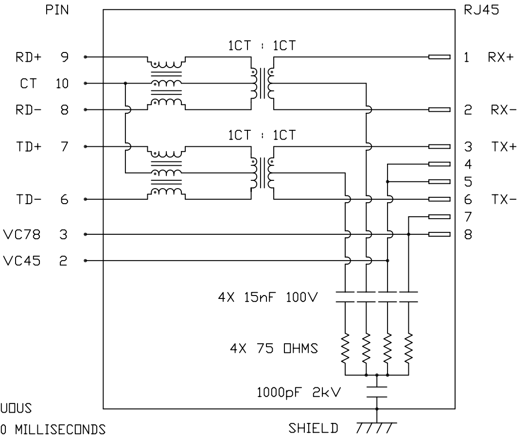
SCHEMATIC
