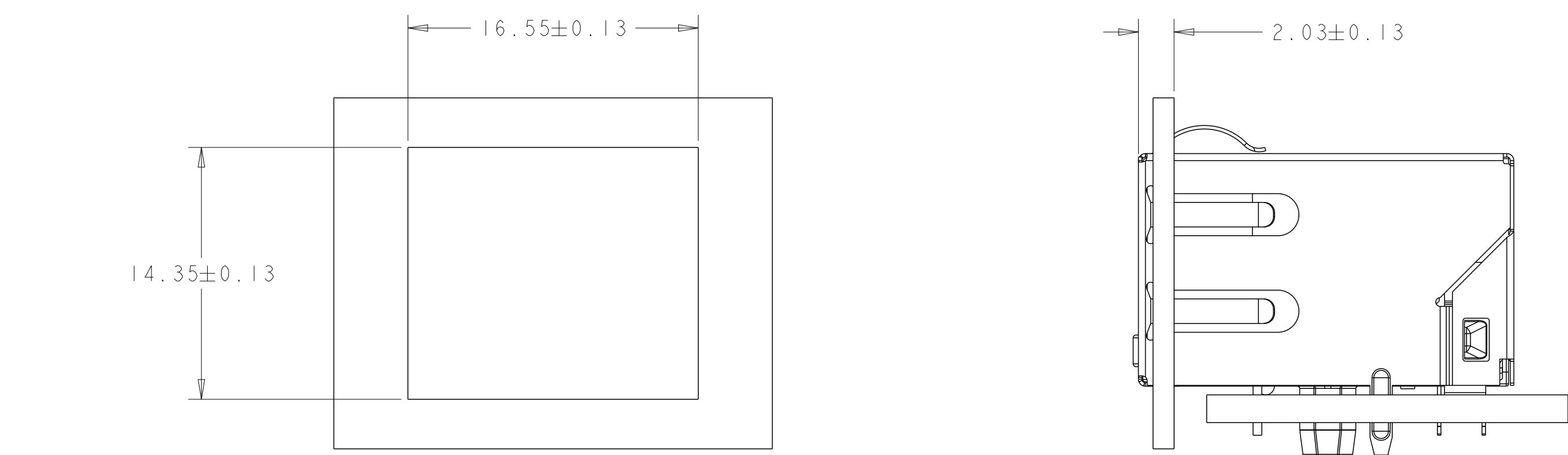
SUGGESTED PANEL OPENING
