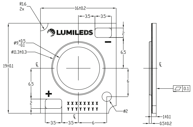
L2C5-xxHG1202E0900, L2C5-xxHG1203E0900
