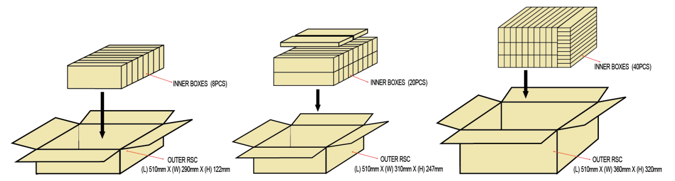
Figure 13. Dimensions for outer box packaging for LUXEON CoB Core Range with CrispColor Technology.
