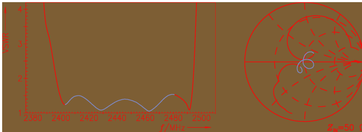
Figure 5: Reflection coefficient at IN port.
