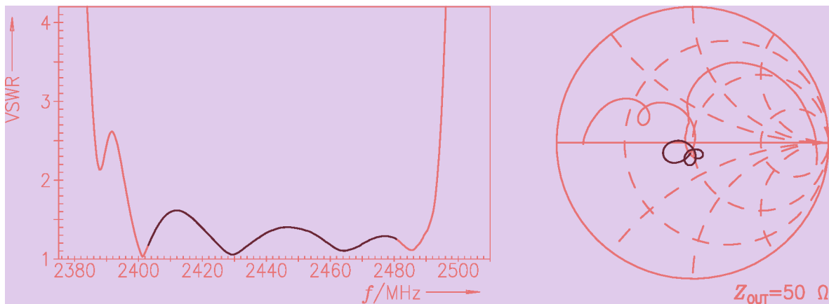
Figure 6: Reflection coefficient at OUT port.
