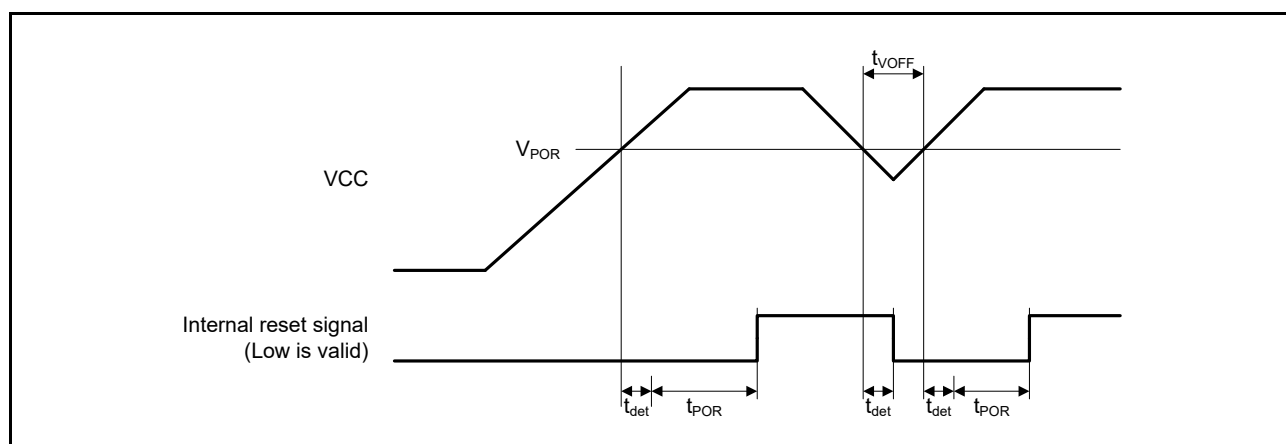
Figure 2.67 Power-on Reset Timing
