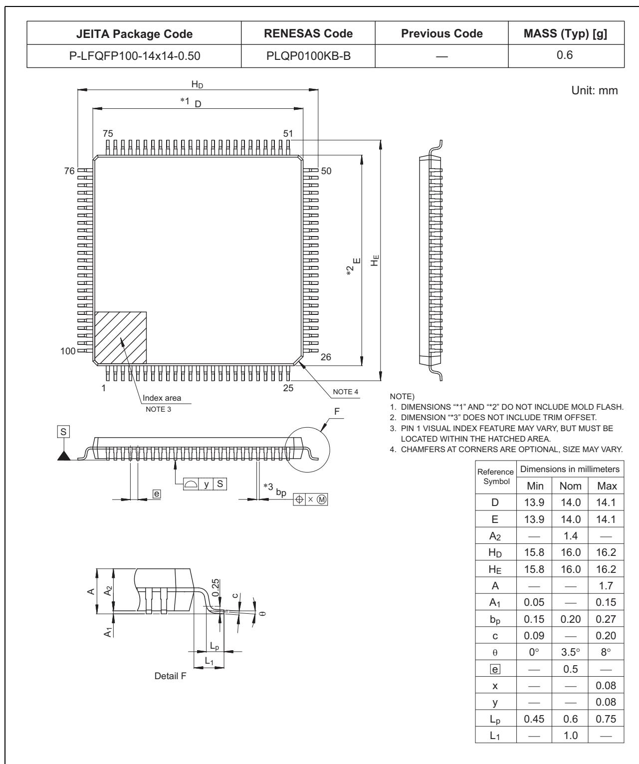
Figure B 100-Pin LFQFP (PLQP0100KB-B)
