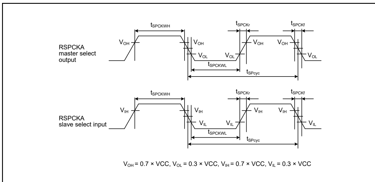
Figure 2.53 RSPCKA Clock Timing
