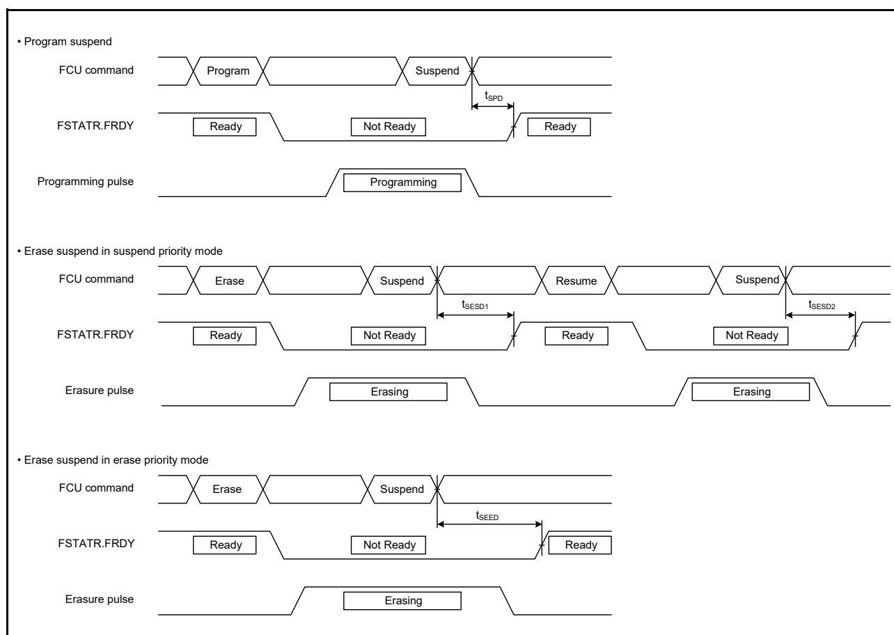
Figure 2.72 Flash Memory Program/Erase Suspend Timing
