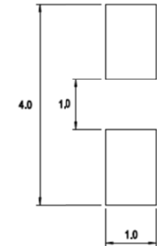
Figure 7 Recommended Soldering Land Pattern
