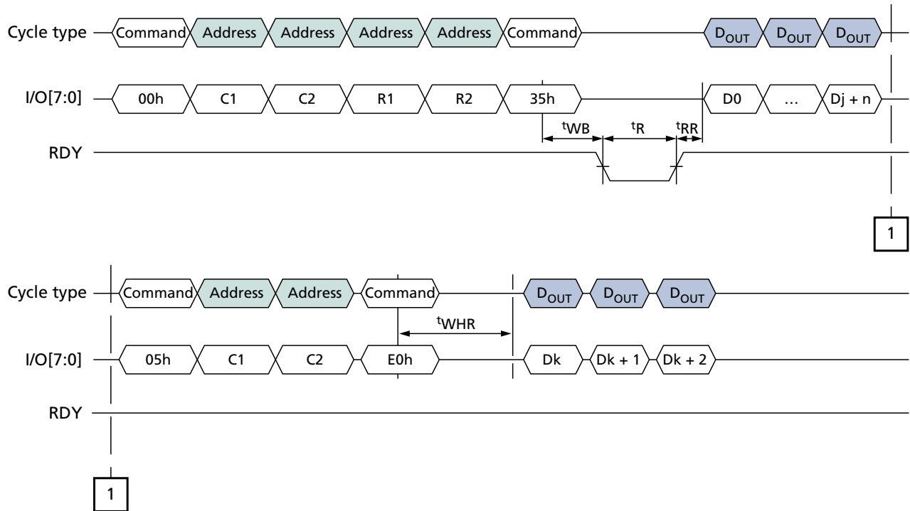
Figure 49: READ FOR INTERNAL DATA MOVE (00h-35h) with RANDOM DATA READ (05h-E0h)
