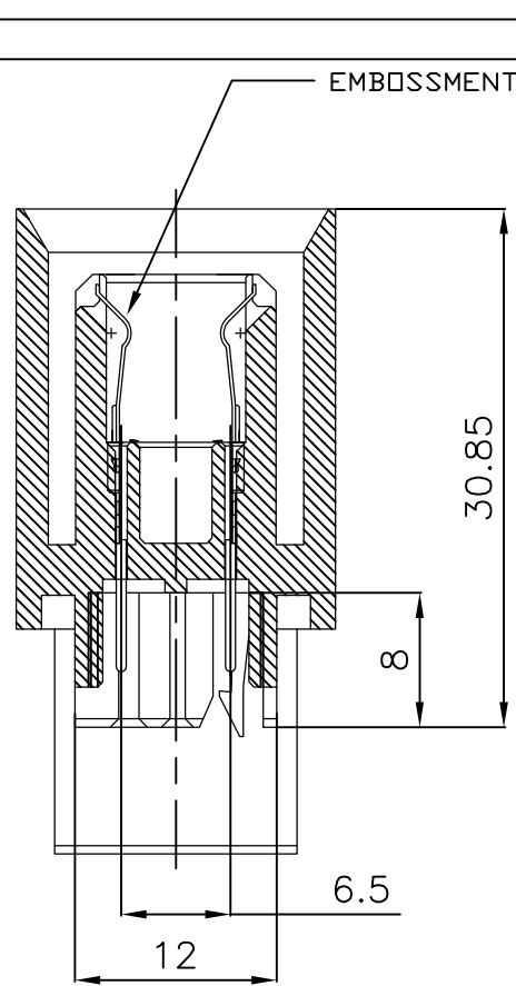
SIGNAL SECTION SECTION B-B
