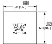
MOUNTING PANEL OPENING (2) UNITS
