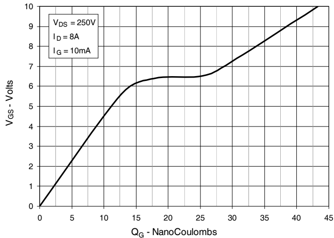
Fig. 9. Gate Charge
