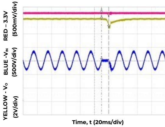
Figure 7. Ride Through at full load, V_{IN} = 230V_{ac} , V_O = 12V_{dc}
