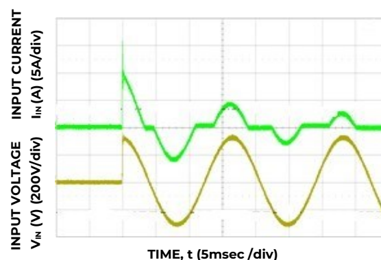
Figure 2. Inrush Current ( V_{IN} = 230V_{ac} , 100% load)
