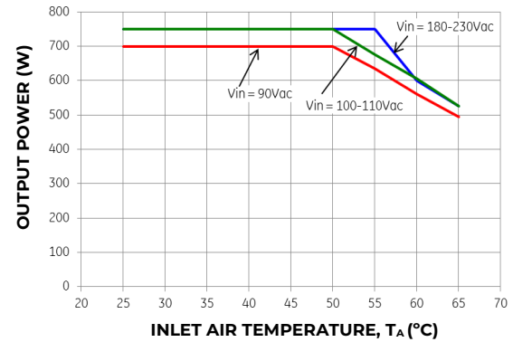
Figure 14. Derating output current versus ambient temperature (Reverse airflow direction)
