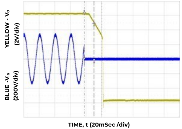
Figure 8. Hold up at 50A load, V_{IN} = 230V_{ac} , V_O = 12V_{dc}
