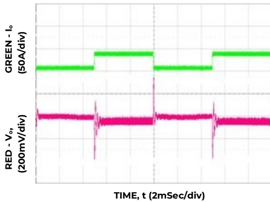
Figure 9. 10%-60%-10% Load Transient, Slew Rate = 1A/\mu S , V_{IN} = 230V_{ac} , V_O = 12V_{dc}
