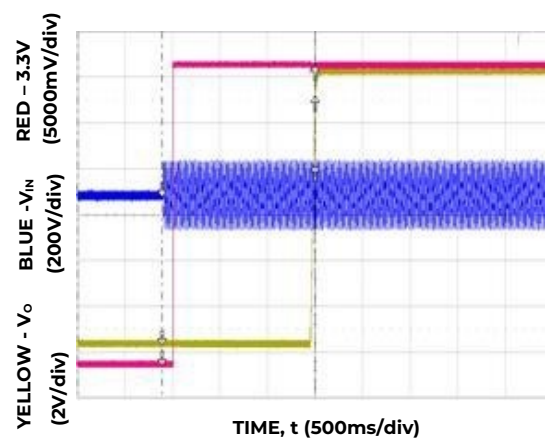
Figure 6. Typical Start-up ( V_{IN} = 150V_{ac} )
