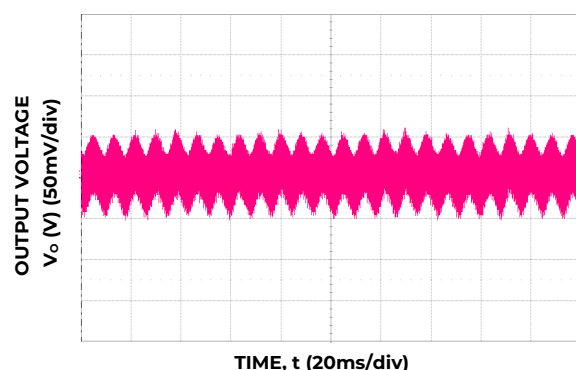
Figure 3. Typical 12V output ripple and noise ( V_{IN} = 230V_{ac} , 100% load).
