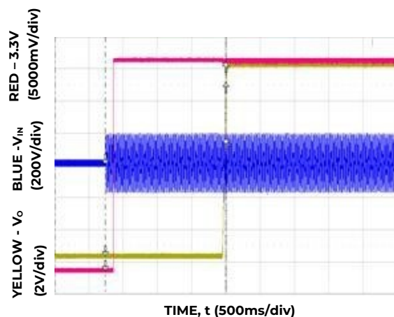
Figure 5. Typical Start-up ( V_{IN} = 230V_{ac} ).
