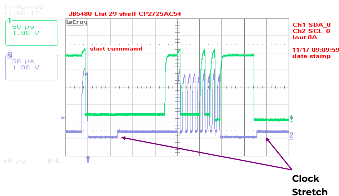
Figure 15. Example waveforms showing clock stretching.
