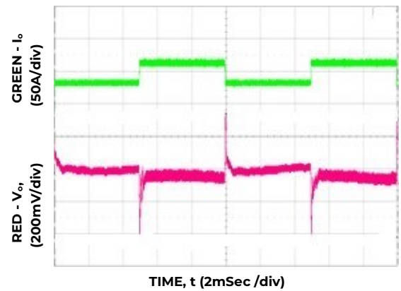
Figure 10. 50%-100%-50% Load Transient, Slew Rate = 1A/\mu S , V_{IN} = 230V_{ac} , V_O = 12V_{dc}
