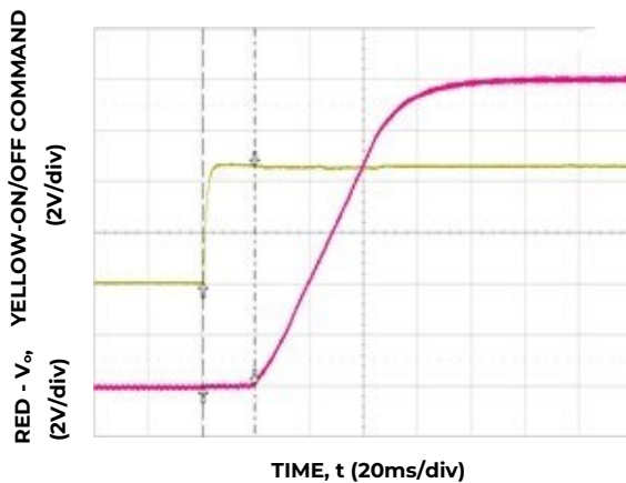
Figure 11. 12V_{dc} Turn-on delay upon inception of ON/ OFF command, V_{in} = 230V
