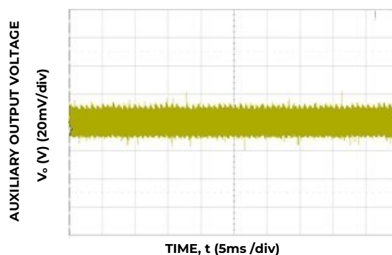
Figure 4. Typical auxiliary 3.3V output ripple and noise ( V_{IN} = 230V_{ac} , 100% load).
